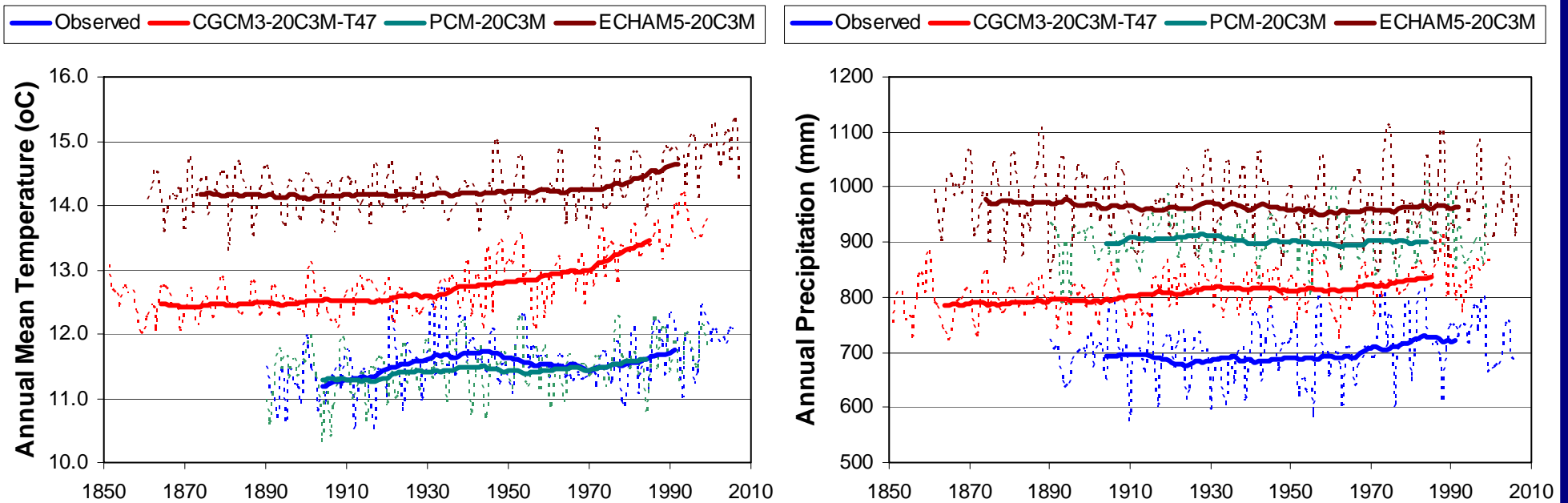
Observed and modelled areal temperature and precipitation, on annual and climatic scales.
